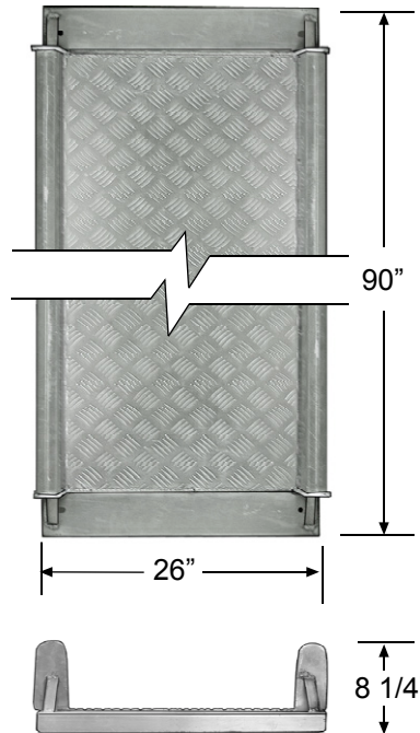
Aluminum Livestock Alleyway
