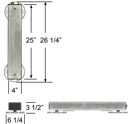
AWB-5 Alleyway Weigh Bars (2)
