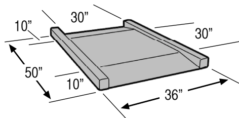
Optional Configuration: Two Ramps
