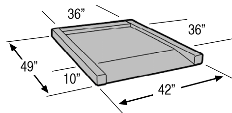
Standard Configuration: One Ramp
